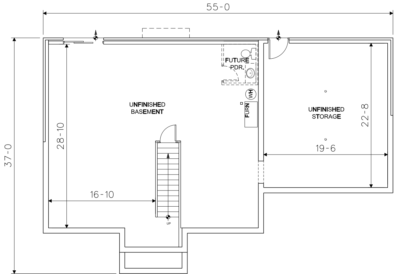
BASEMENT PLAN
